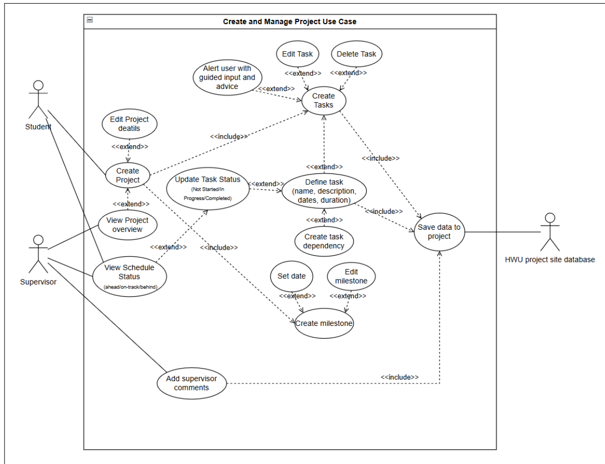
Fig. 3. Create and Manage Project Use Case Diagram.
